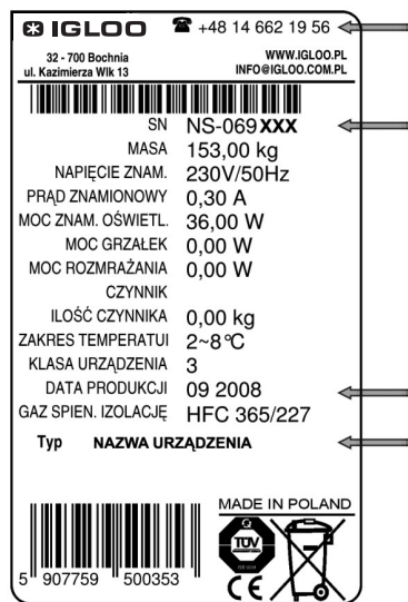
Fig.13 Data plate
