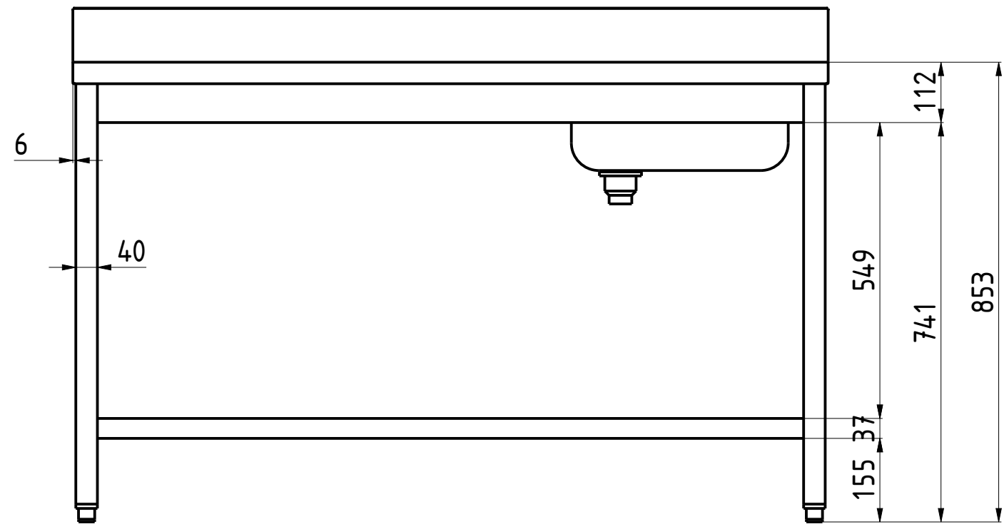
FRONT VIEW 1:10
