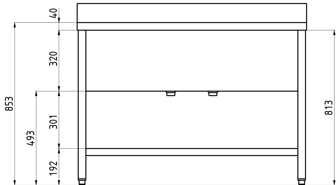
FRONT VIEW 1:10
