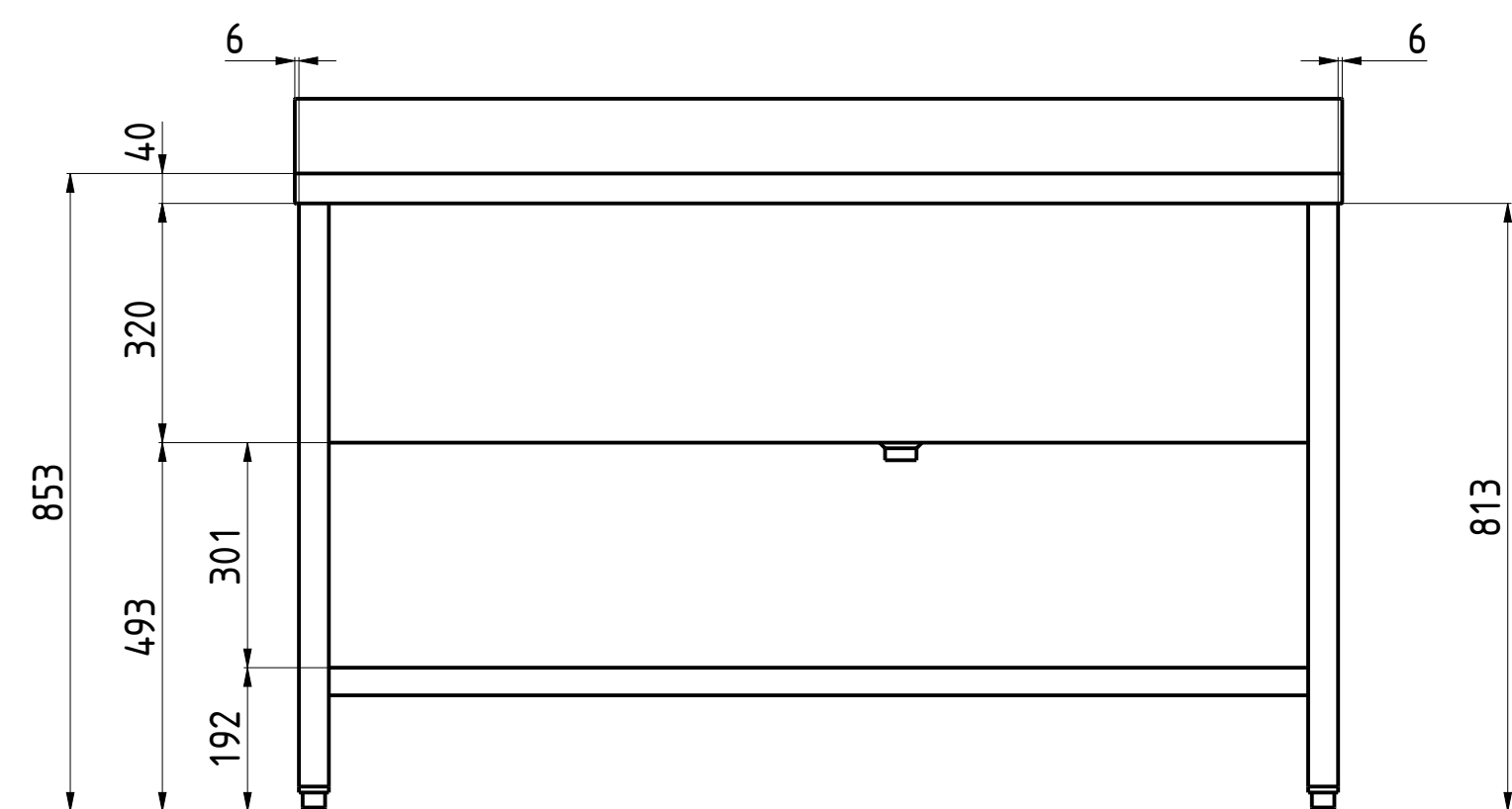
FRONT VIEW 1:10
