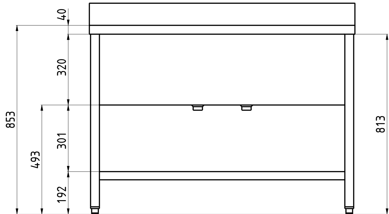
FRONT VIEW 1:10
