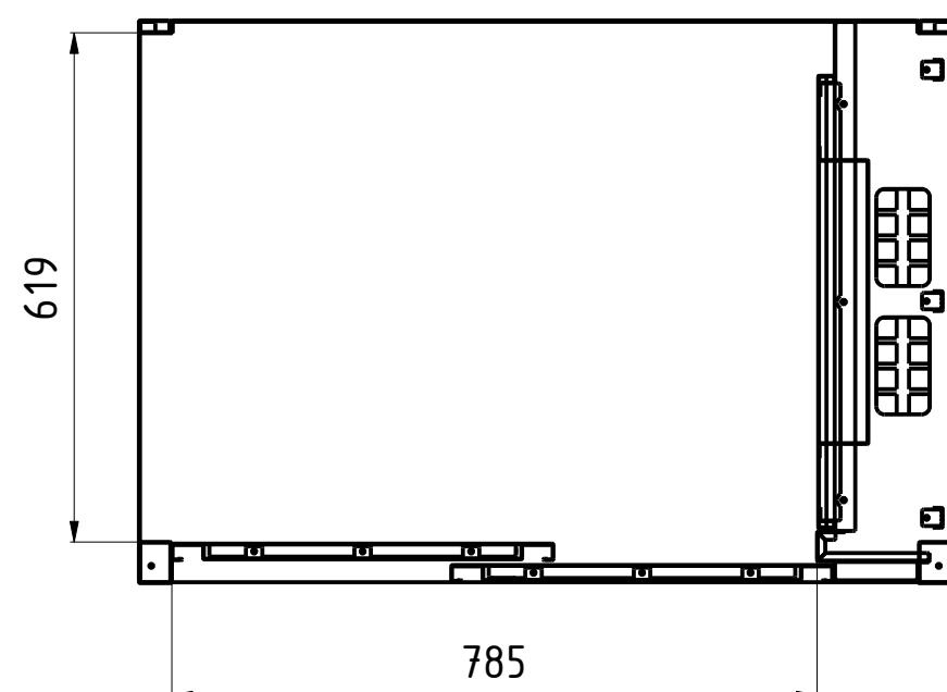
INTERNAL DIM D-D
