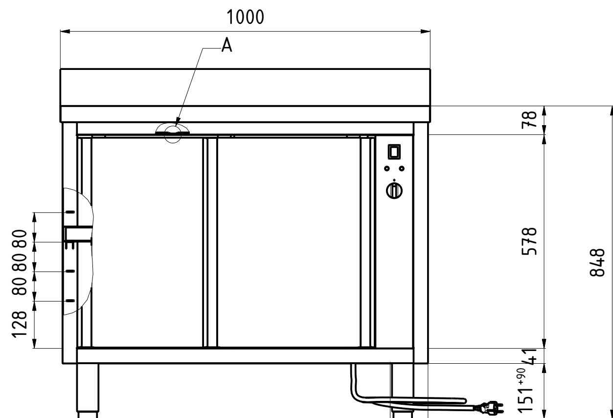
FRONT VIEW 102* B-B C-C 1:10
