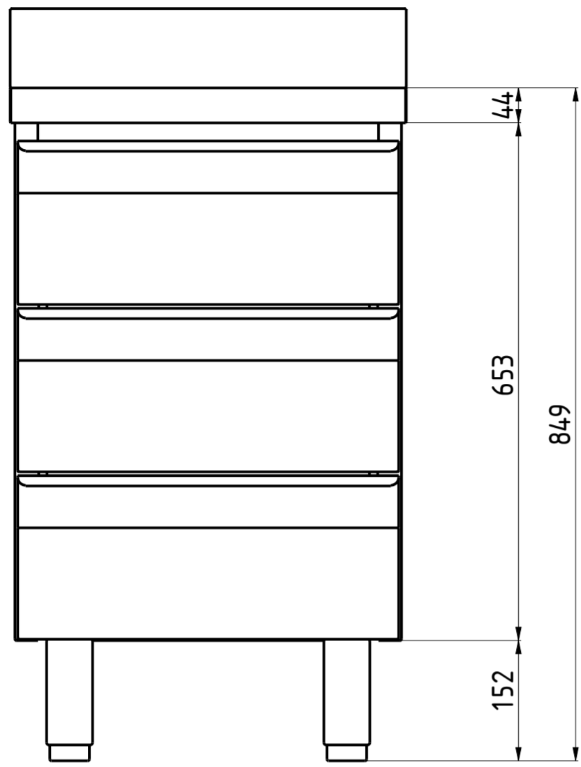
FRONT VIEW 3:20
