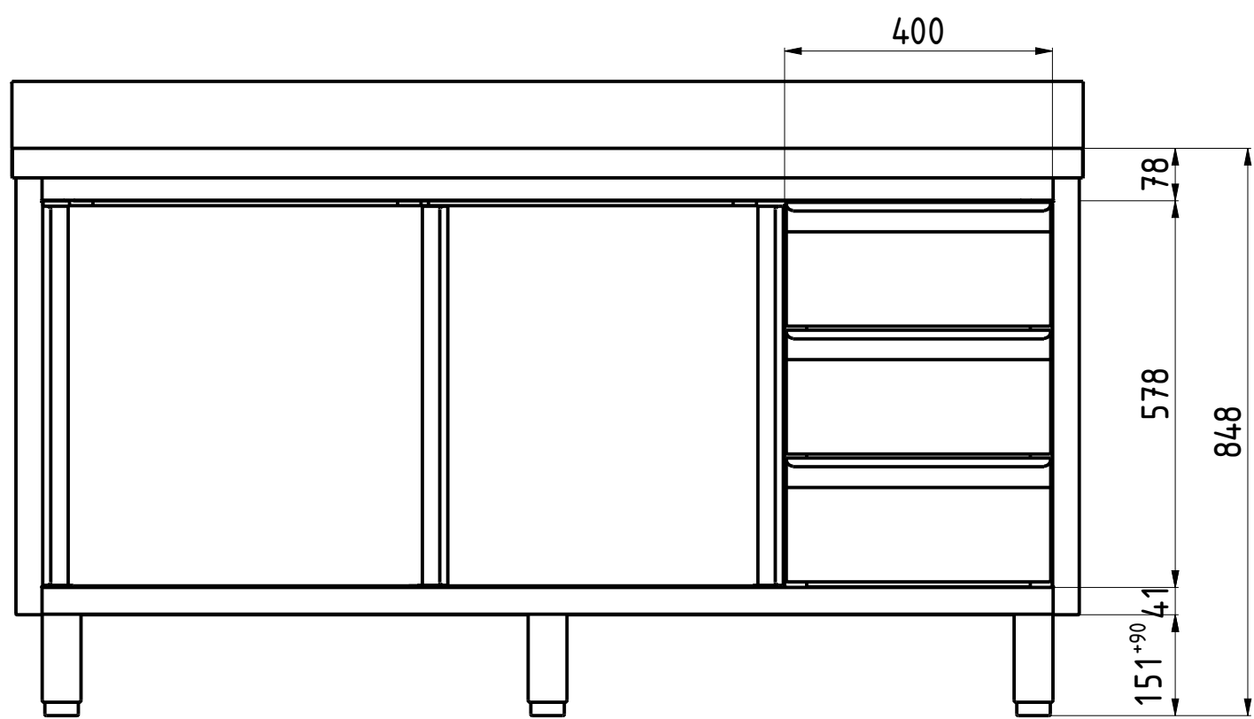
FRONT VIEW 1:10
