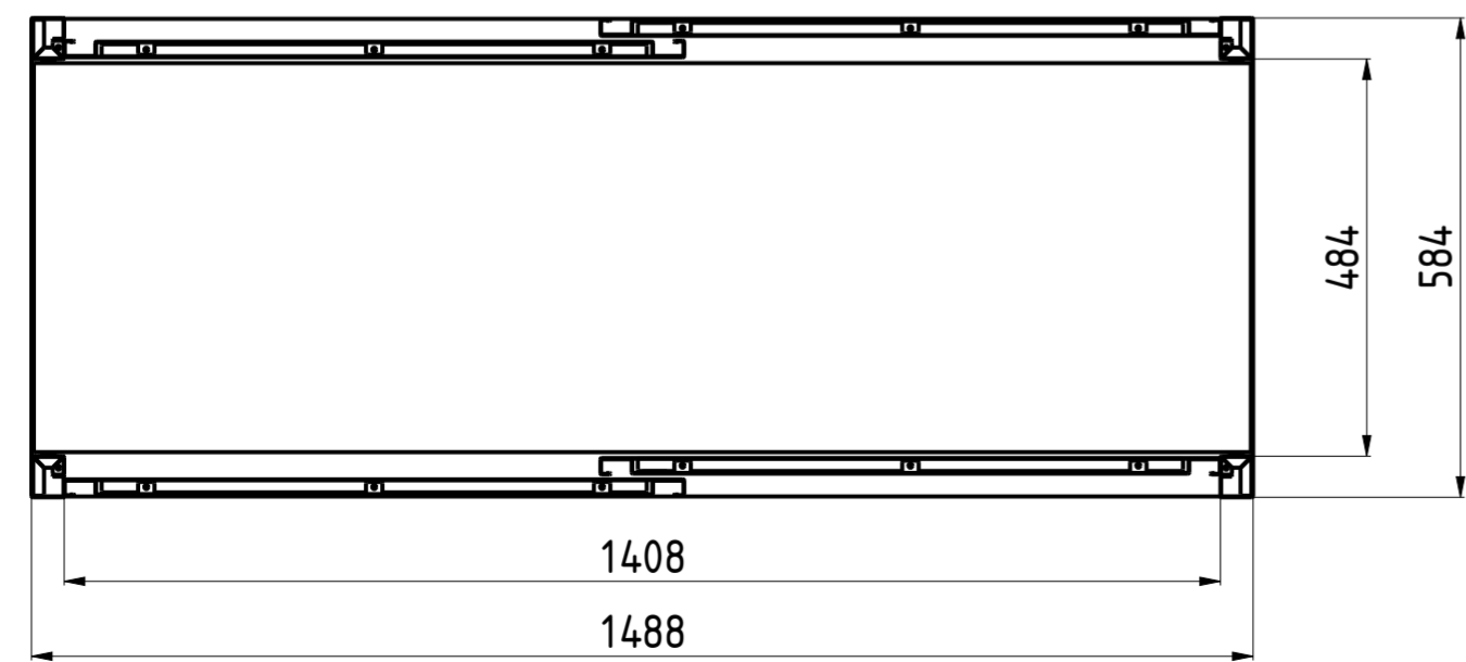
INTERNAL DIM C-C
