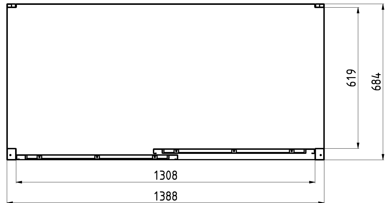
INTERNAL DIM D-D
