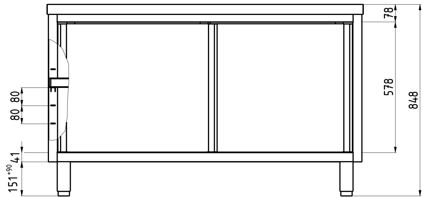
FRONT VIEW C-C 1:10
