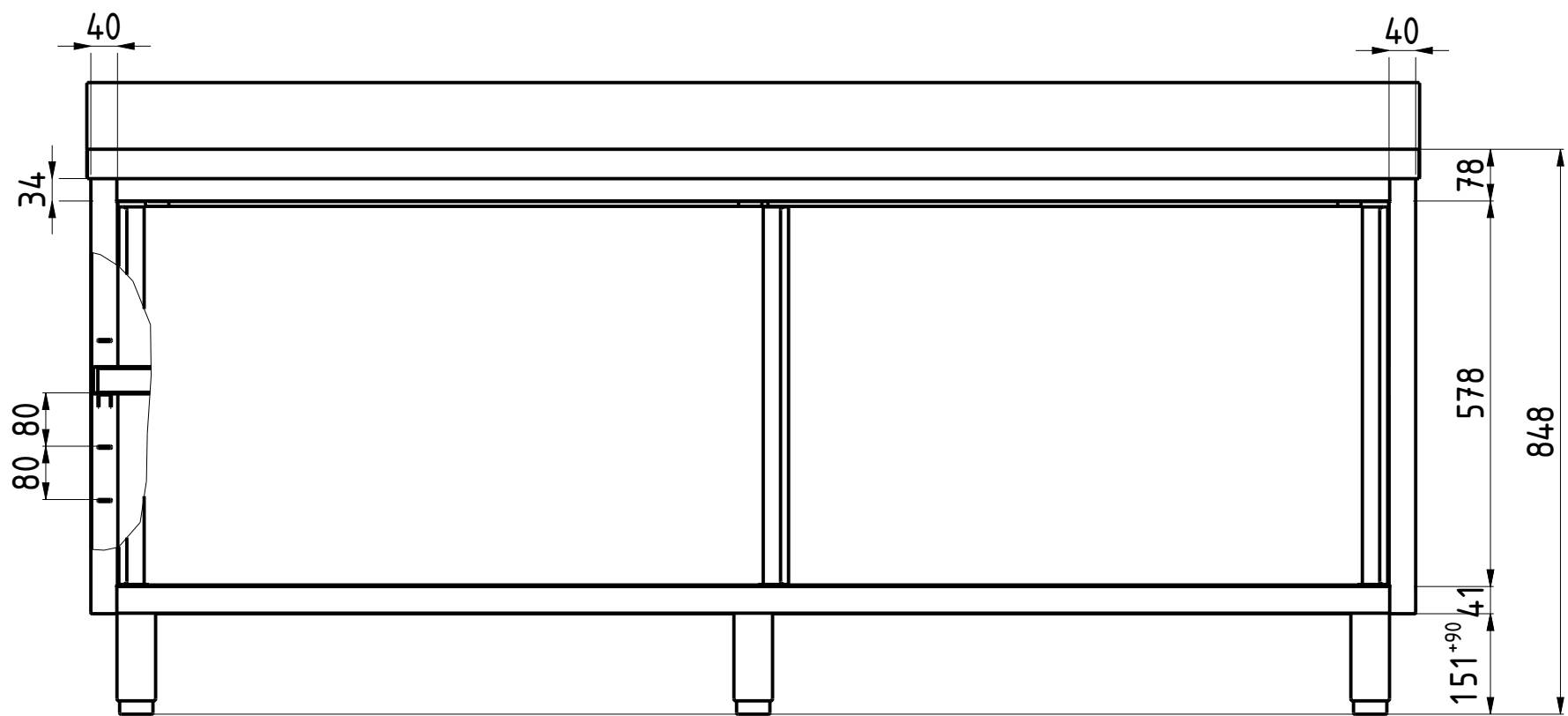
FRONT VIEW C-C 1:10
