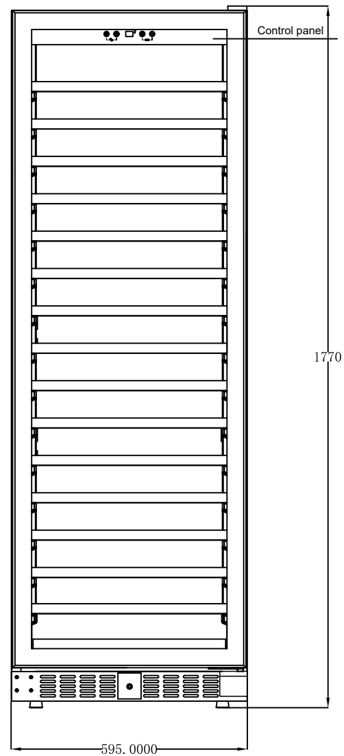
Vino 481 outline drawing - Front
