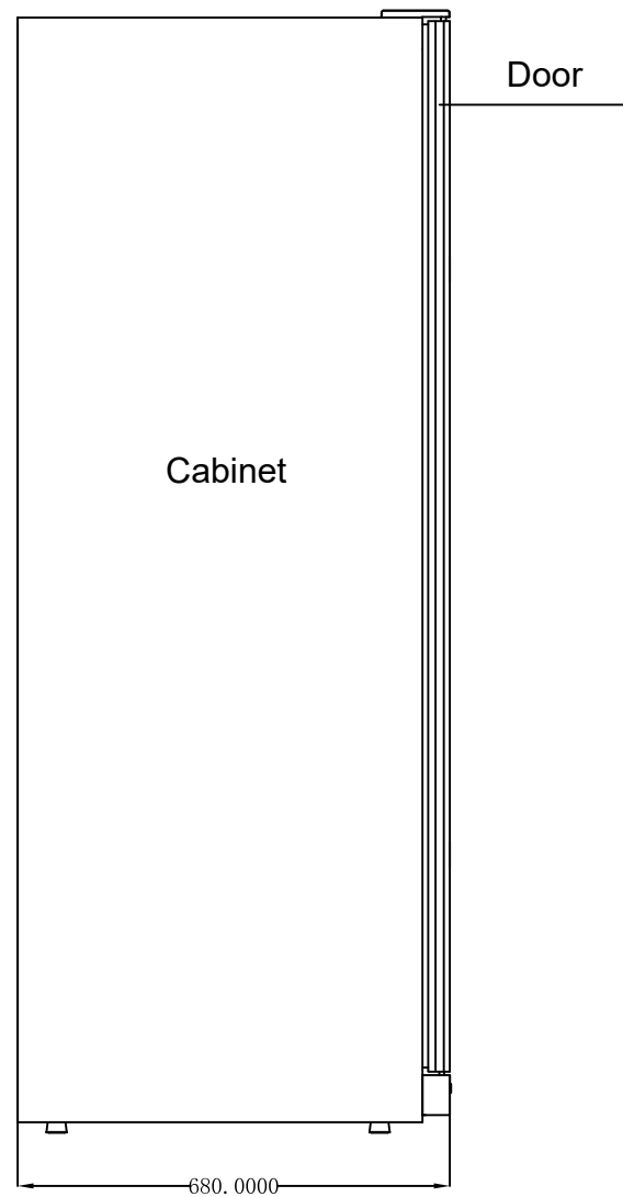
Vino 481 outline drawing - Side
